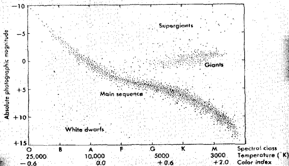
Fig. 6. The Hertzsprung-Russell diagram for stars of known distance. A diagram such as this is indicative of the present evolutionary status of the stars shown. Apparently supernovae do not occur in stars that are on the main sequence. The sun is located on the main sequence at G5.
