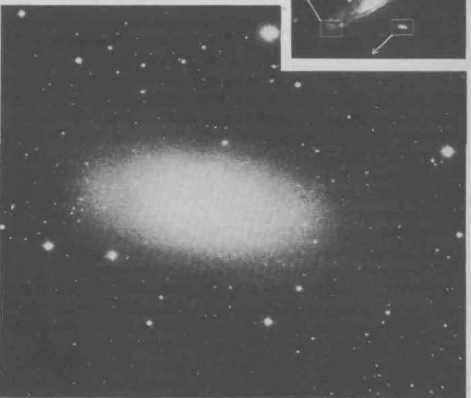
NGC 205, comparison of the Andromeda Nebula, photographed in yellow light shows stars of Population II. The brightest stars are red and 100 times fainter than the blue giants of Population I.
