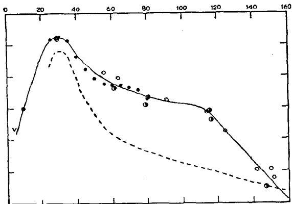
Fig. 2. Supernova light curves. The dashed line represents the typical type I curve whereas the solid line is a composite light curve for three type II supernovae. The points represent the actual measurements made of the light from the three supernovae. The ordinate is photographic magnitude and the abscissa is days. Scales have been shifted to bring the curves into coincidence.
