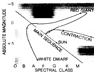
Fig. 7. Evolutionary track followed by a star several times more massive than the sun.
