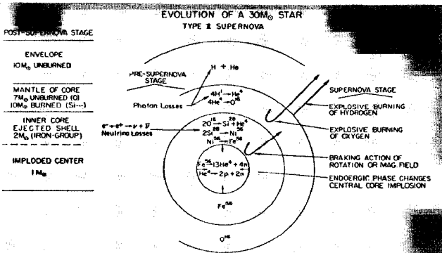
Fig. 9. The evolution of a star 30 times more massive than the sun illustrating the pre-supernova, type II supernova, and post-supernova stages. It is assumed that braking action due to rotation or some other mechanism ultimately leads to mantle-envelope explosion following core implosion caused by endoergic nuclear phase changes. The explosive burning of previously unburned oxygen is taken to be the source of energy of the explosion.
